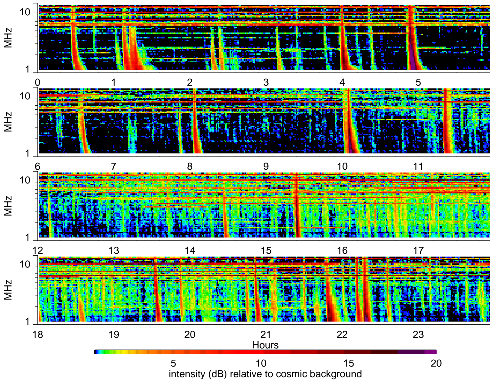
Wind Waves RAD2 receiver: 2000/1/19
