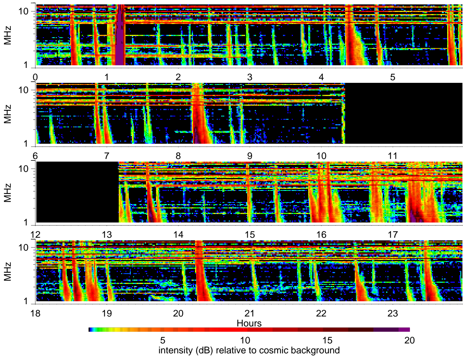
Wind Waves RAD2 receiver: 2000/1/18
