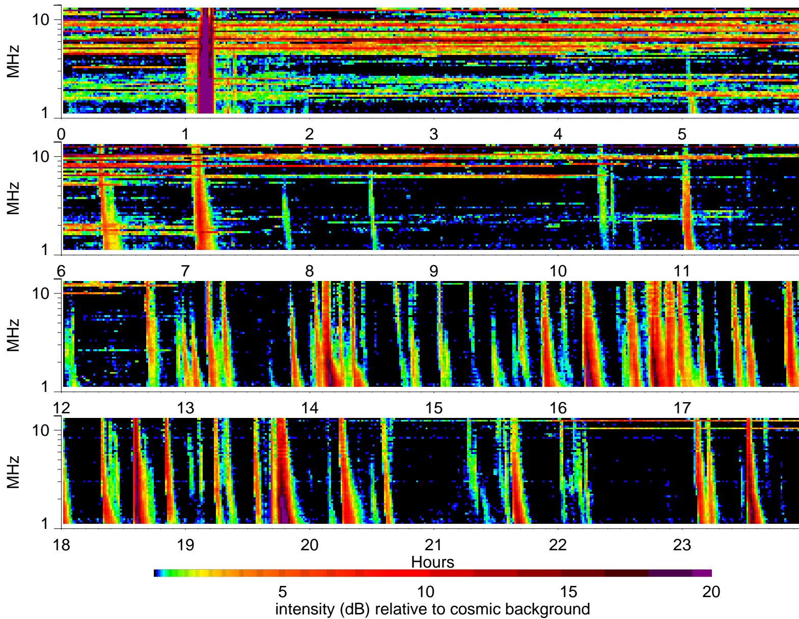
Wind Waves RAD2 receiver: 2000/1/16
