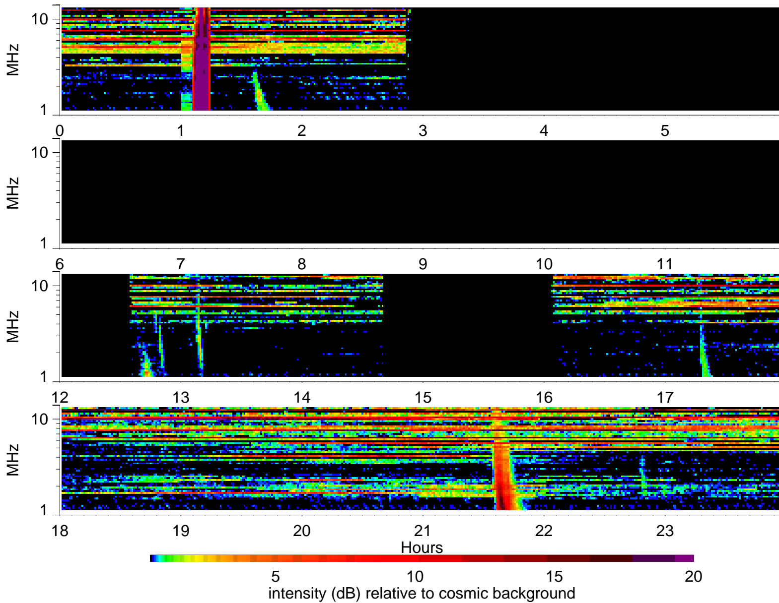
Wind Waves RAD2 receiver: 2000/1/14
