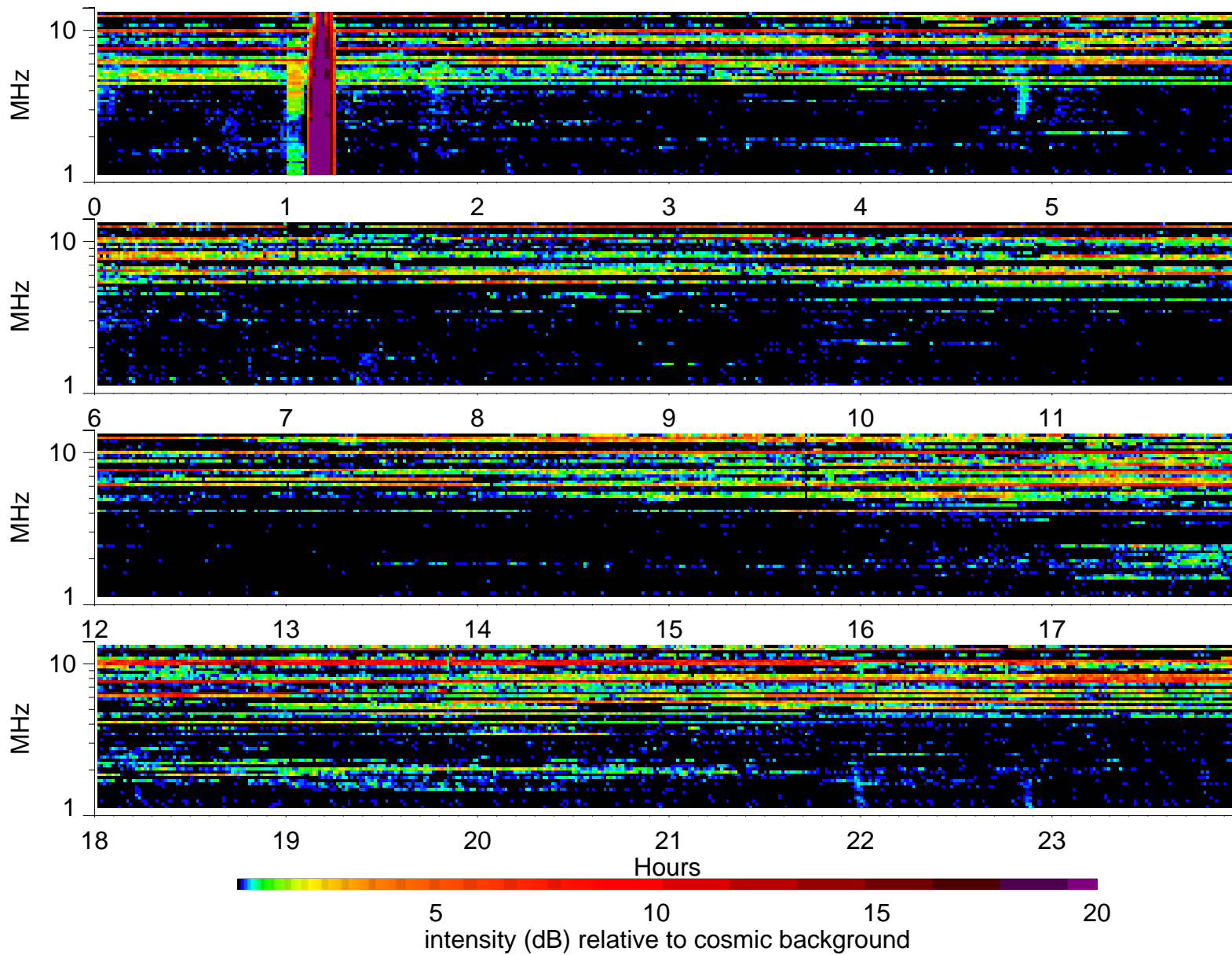
Wind Waves RAD2 receiver: 2000/1/10
