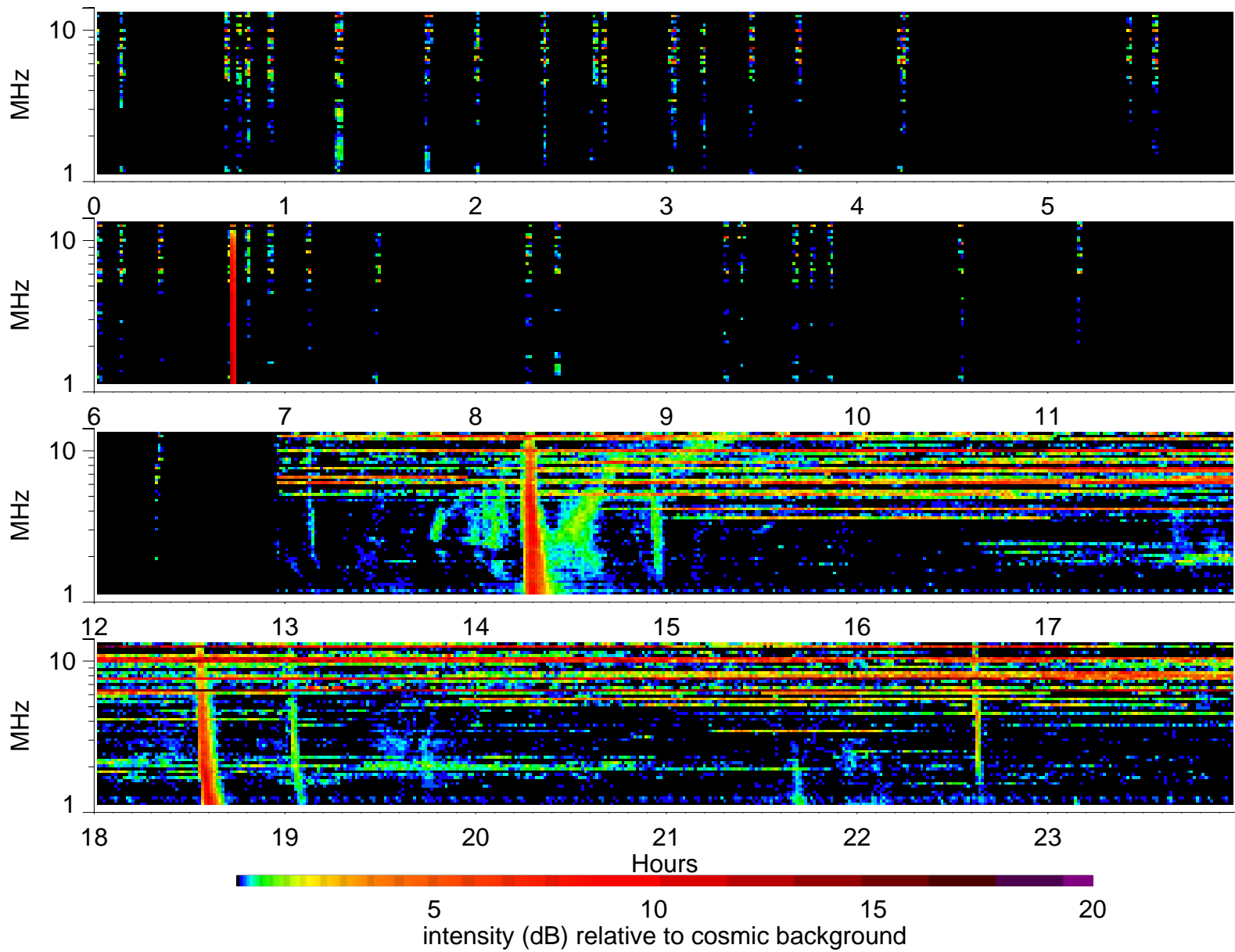
Wind Waves RAD2 receiver: 2000/1/9
