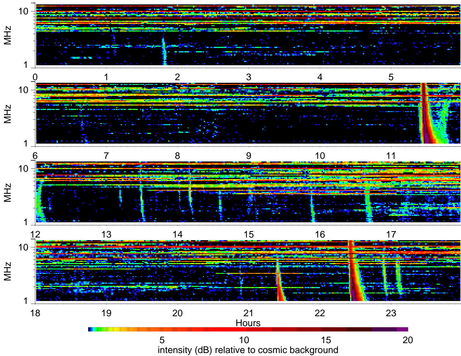
Wind Waves RAD2 receiver: 2000/1/7
