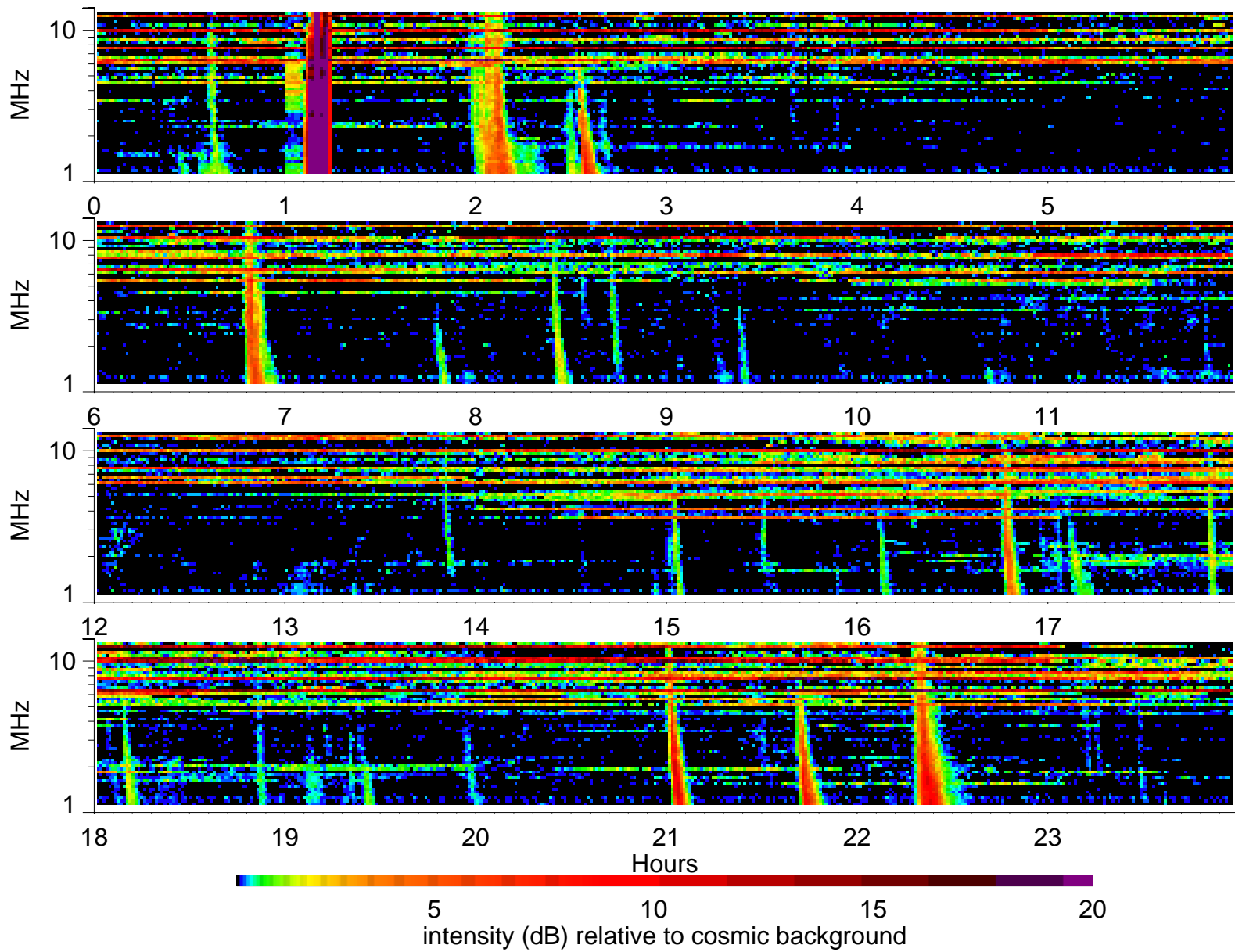
Wind Waves RAD2 receiver: 2000/1/6
