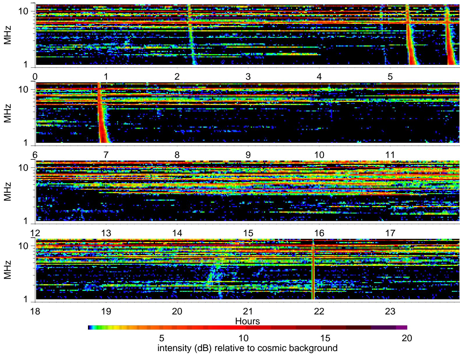
Wind Waves RAD2 receiver: 2000/1/3
