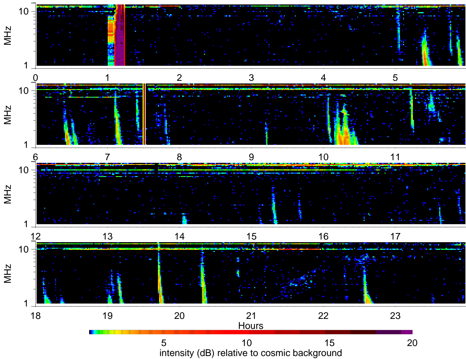
Wind Waves RAD2 receiver: 1998/6/11
