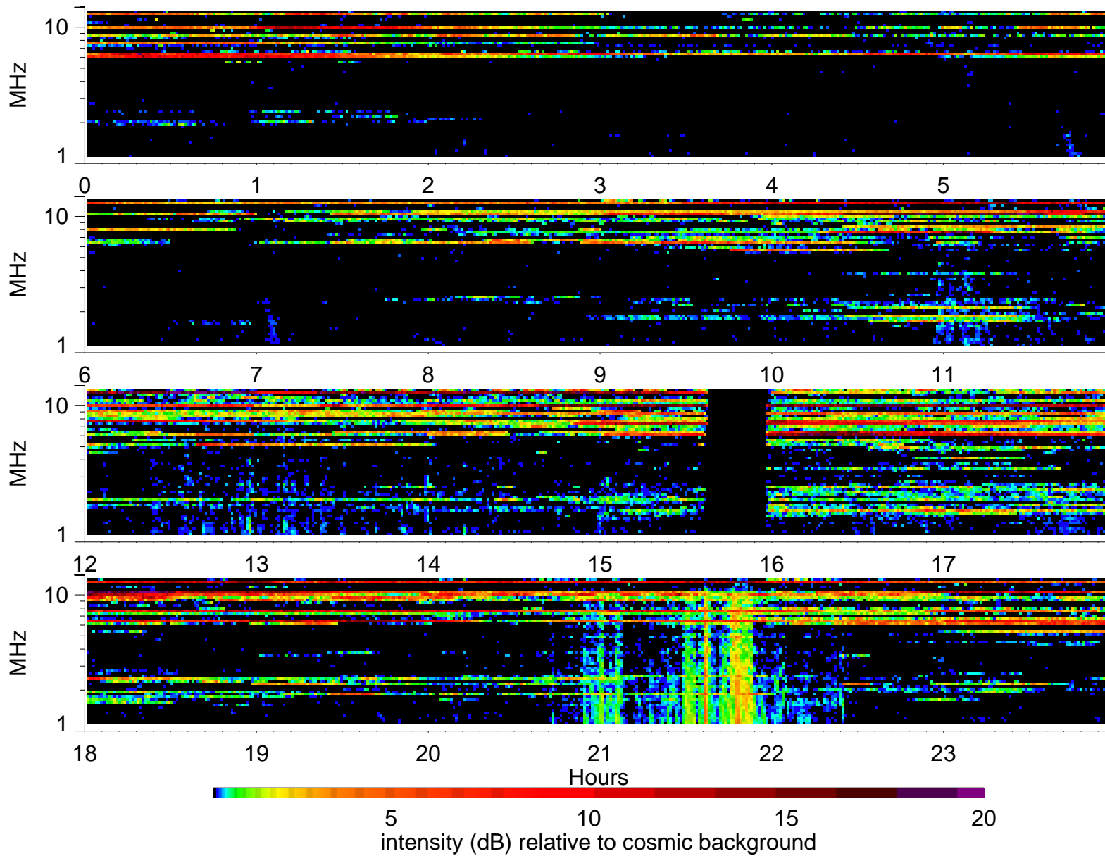
Wind Waves RAD2 receiver: 1996/12/28
