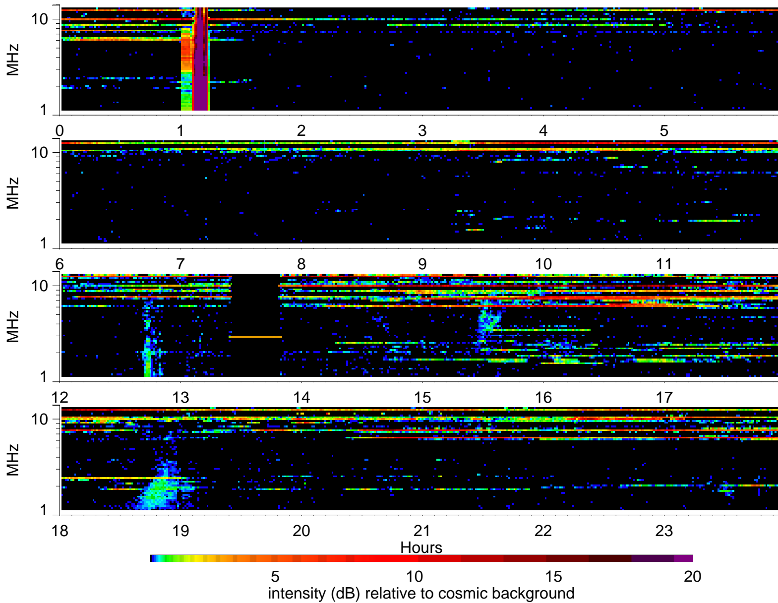
Wind Waves RAD2 receiver: 1996/12/27
