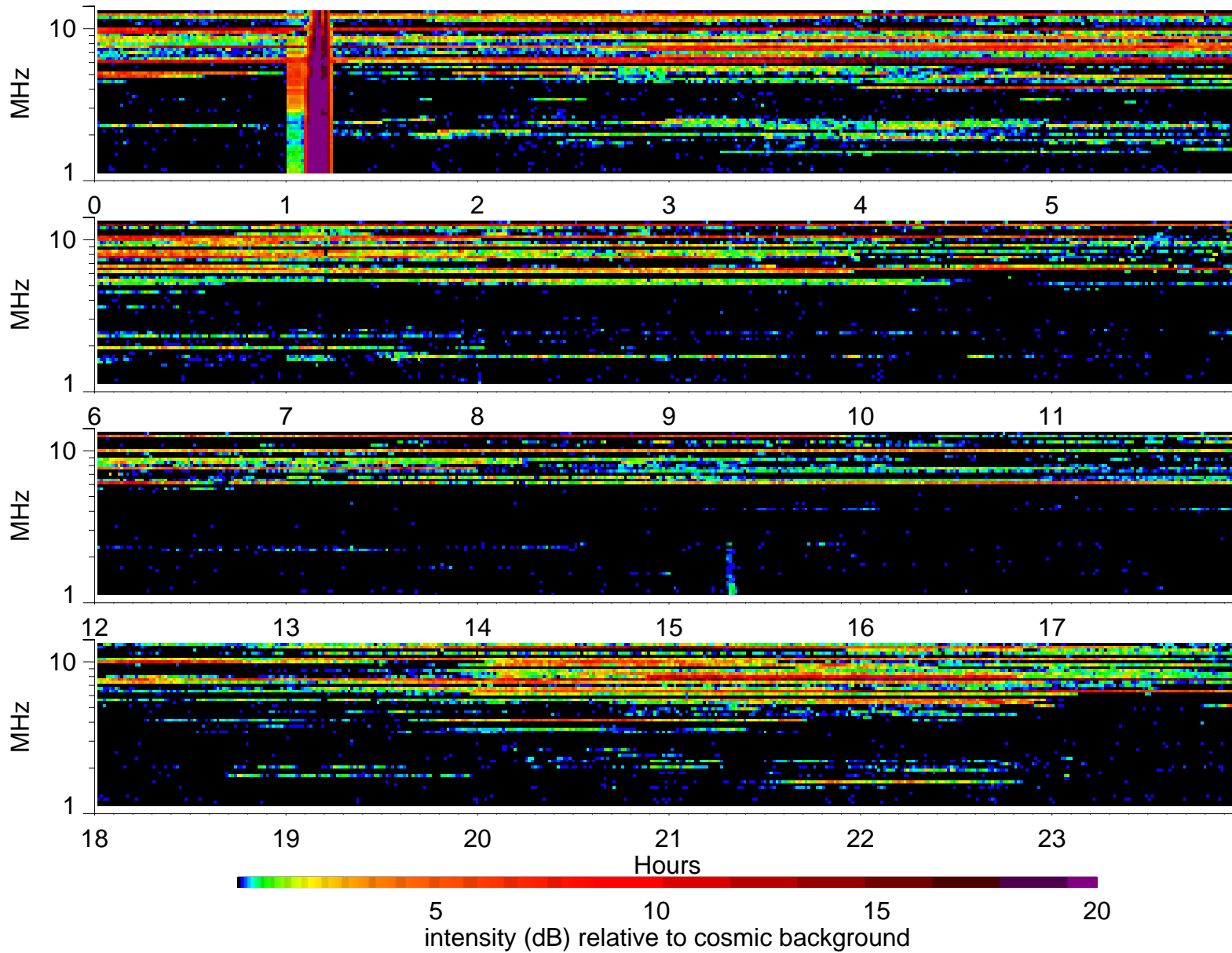
Wind Waves RAD2 receiver: 1996/12/7
