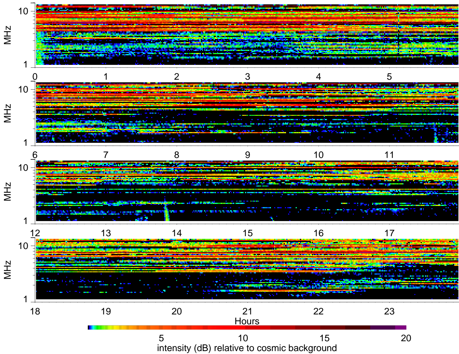
Wind Waves RAD2 receiver: 1996/12/4
