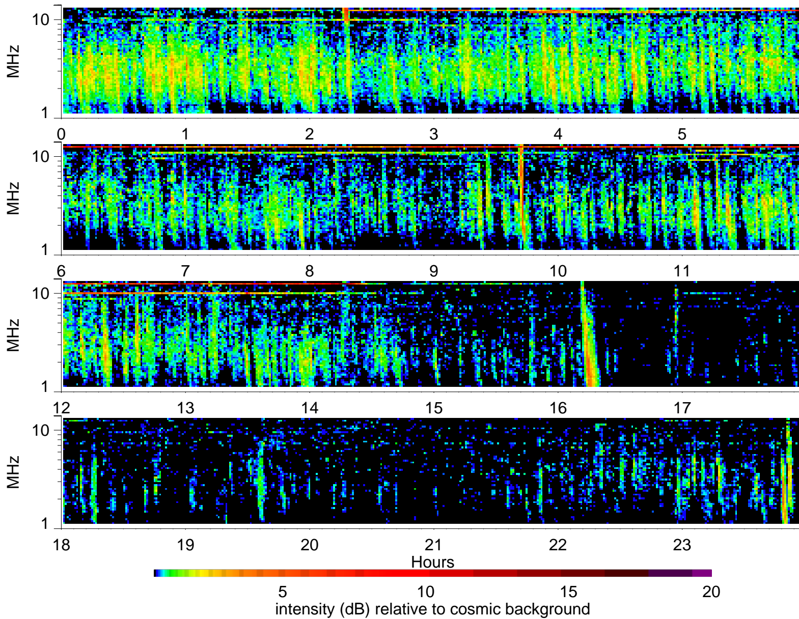
Wind Waves RAD2 receiver: 1996/11/28
