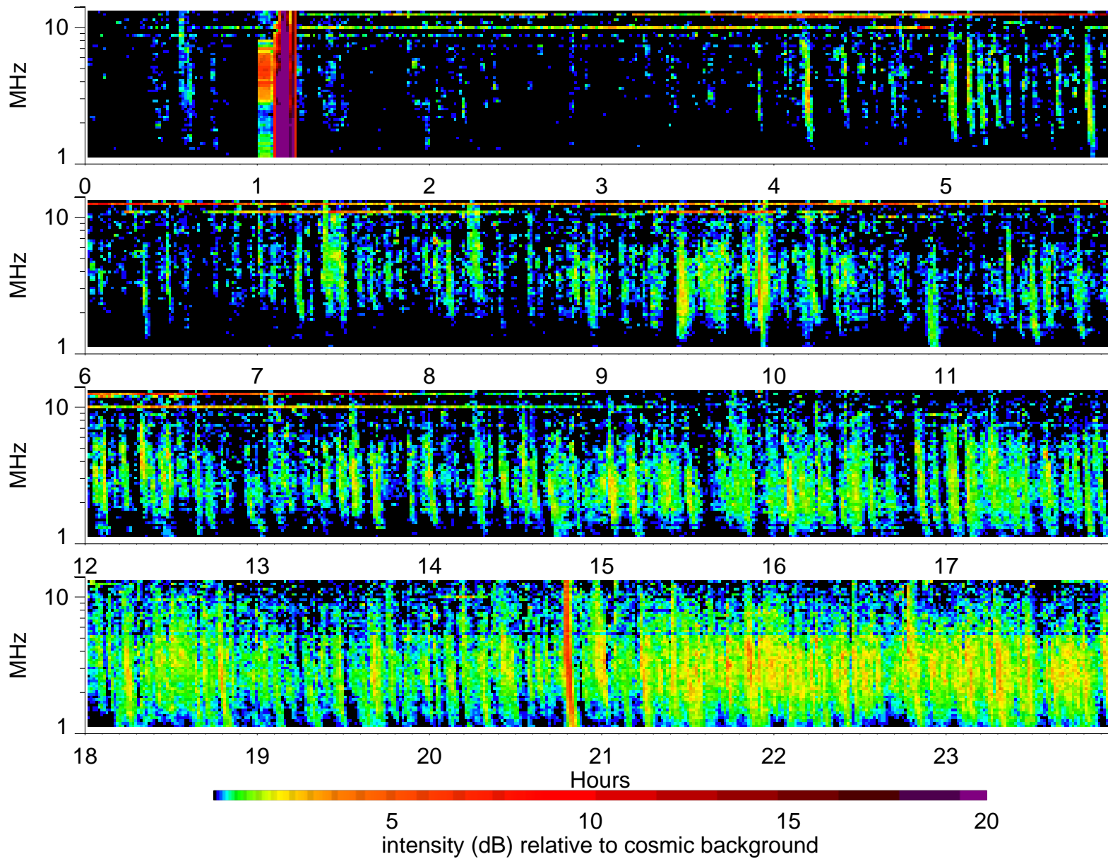
Wind Waves RAD2 receiver: 1996/11/27
