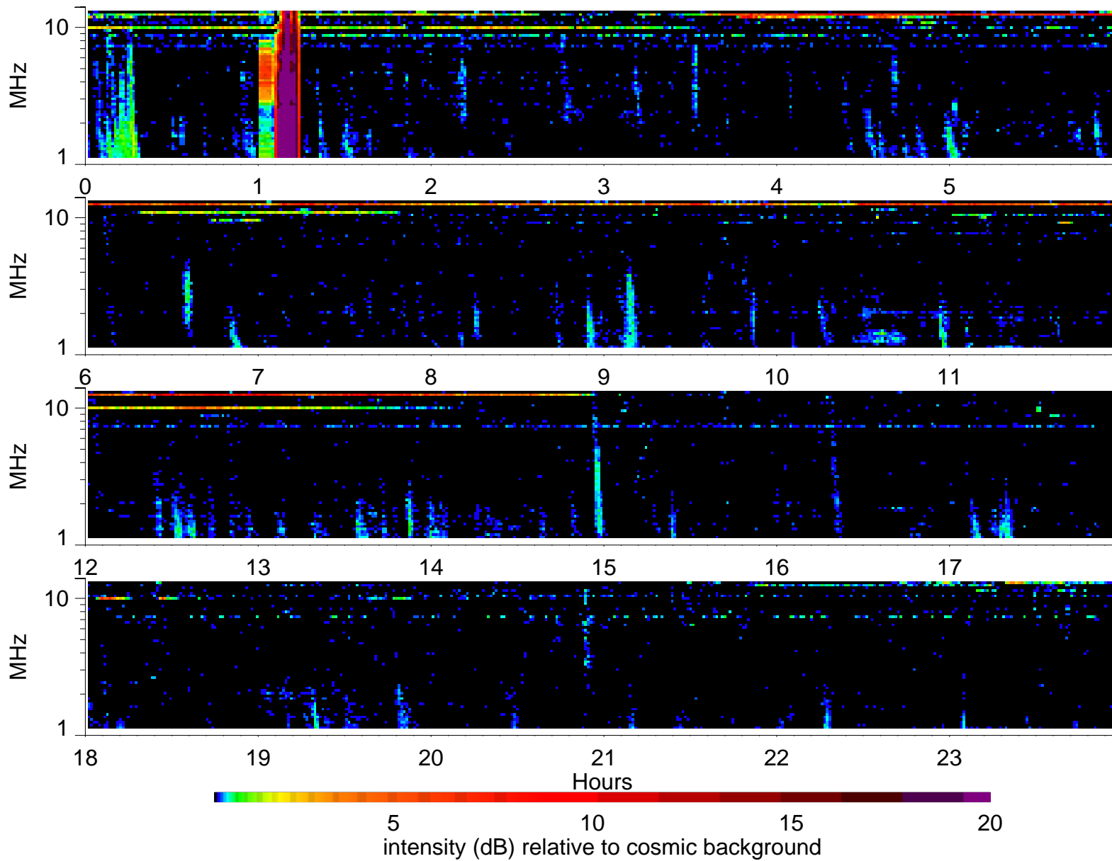
Wind Waves RAD2 receiver: 1996/11/25
