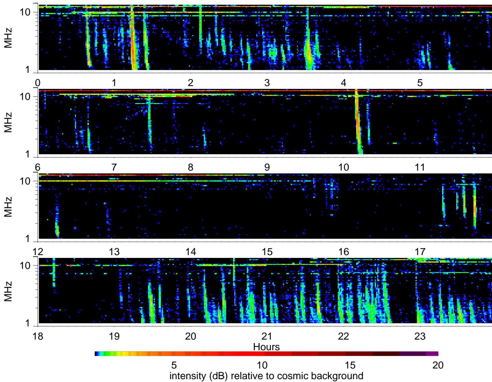
Wind Waves RAD2 receiver: 1996/11/24
