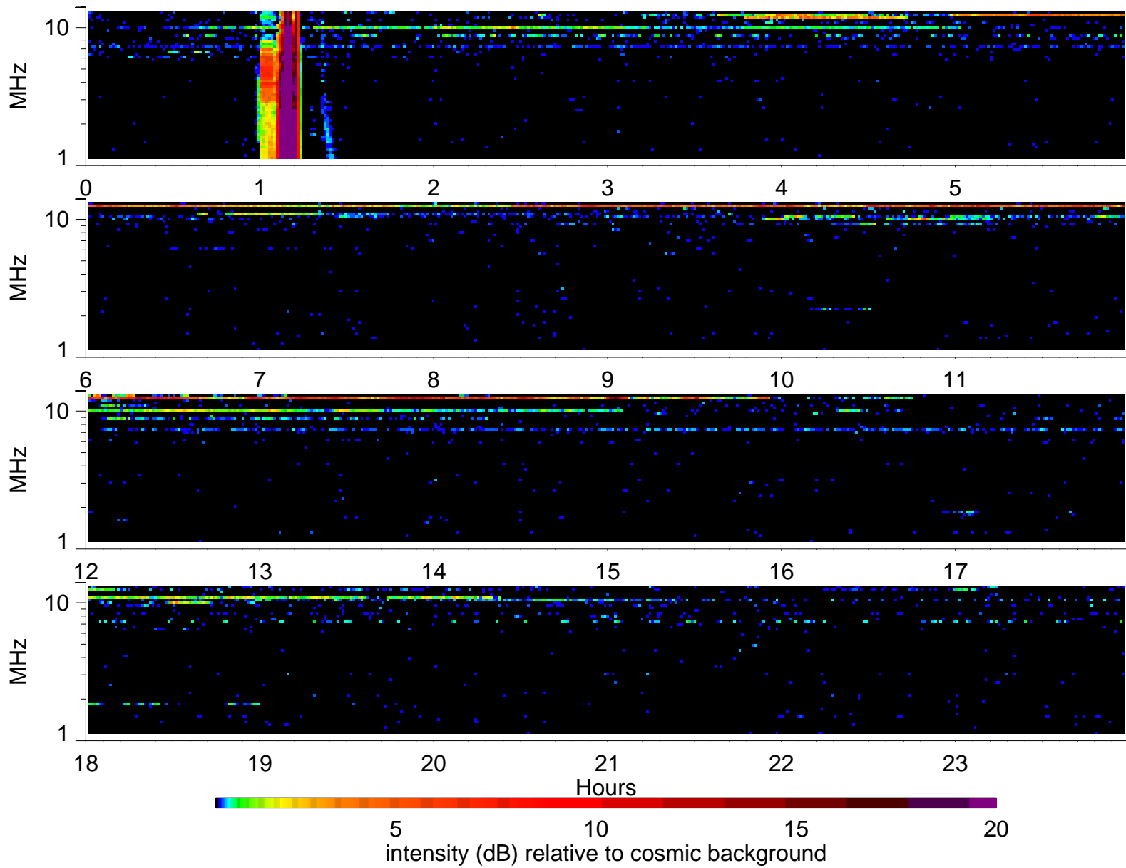
Wind Waves RAD2 receiver: 1996/11/11
