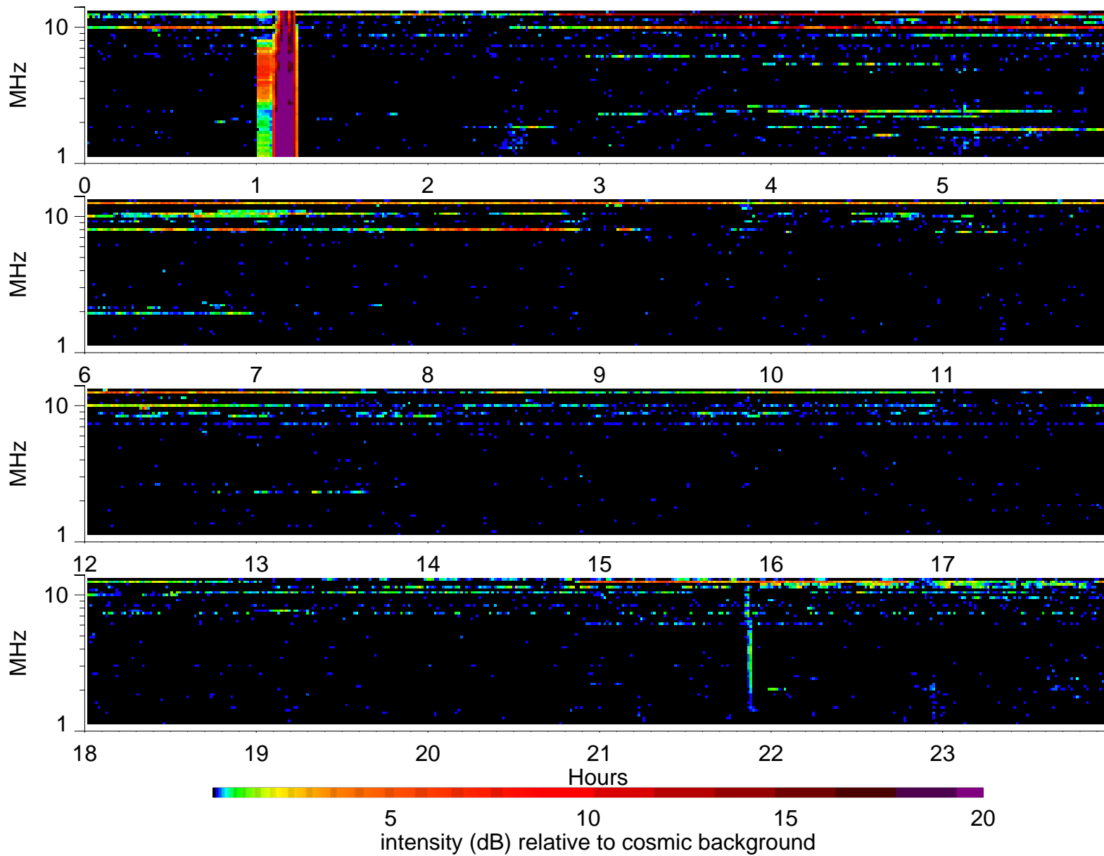
Wind Waves RAD2 receiver: 1996/10/26
