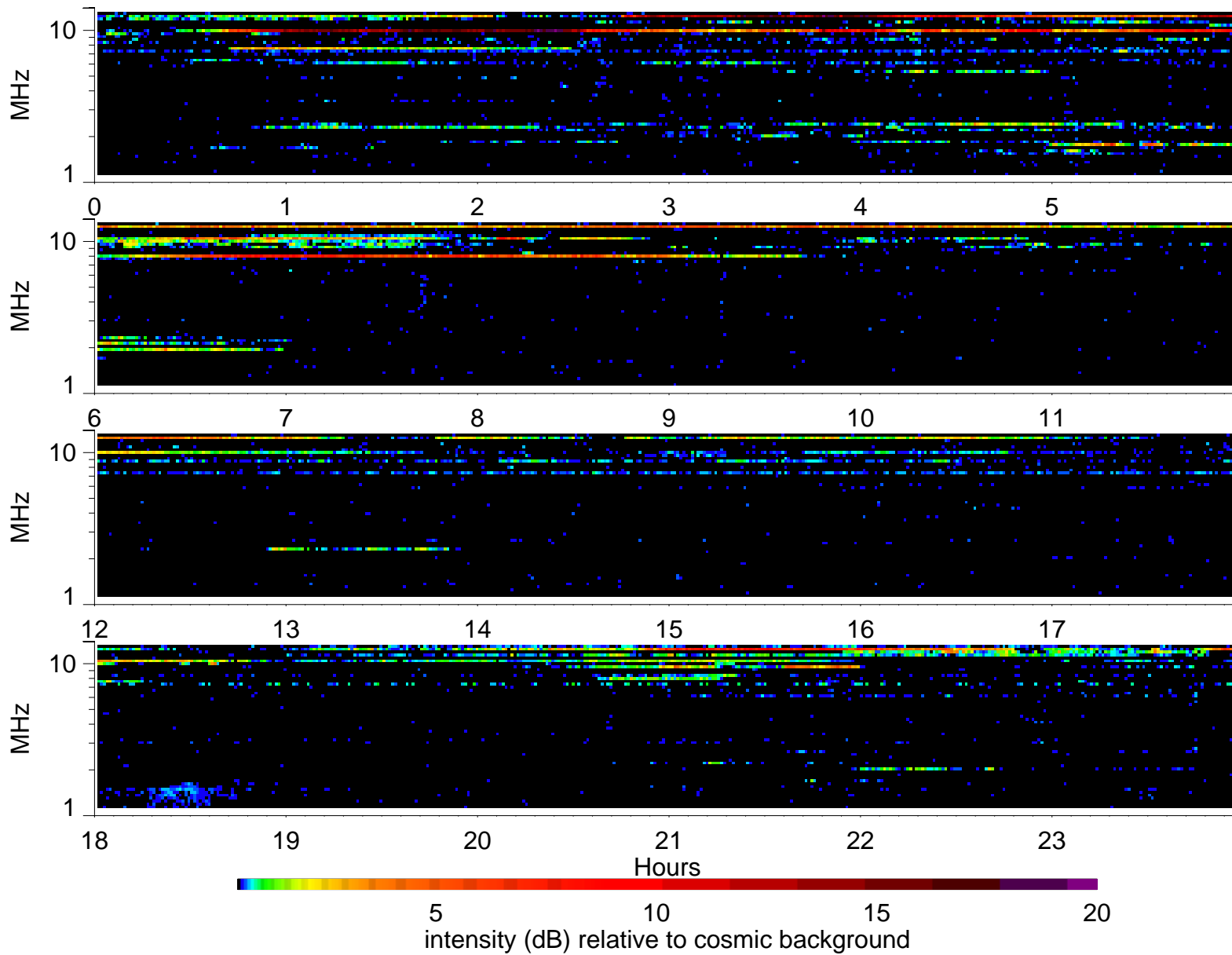
Wind Waves RAD2 receiver: 1996/10/25
