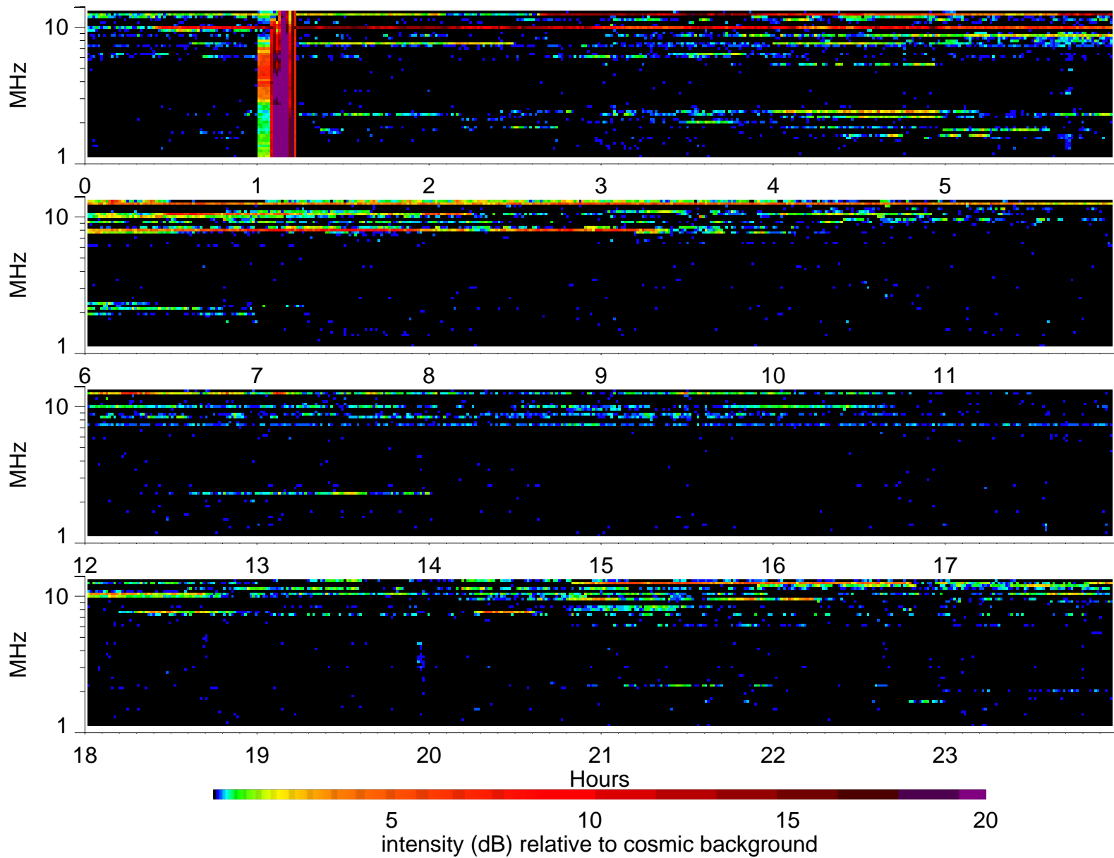
Wind Waves RAD2 receiver: 1996/10/24
