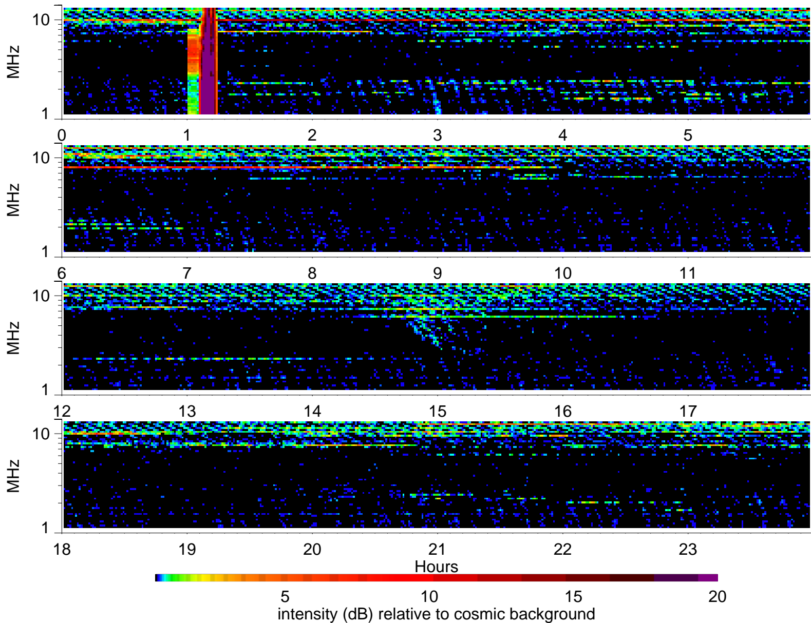
Wind Waves RAD2 receiver: 1996/10/22
