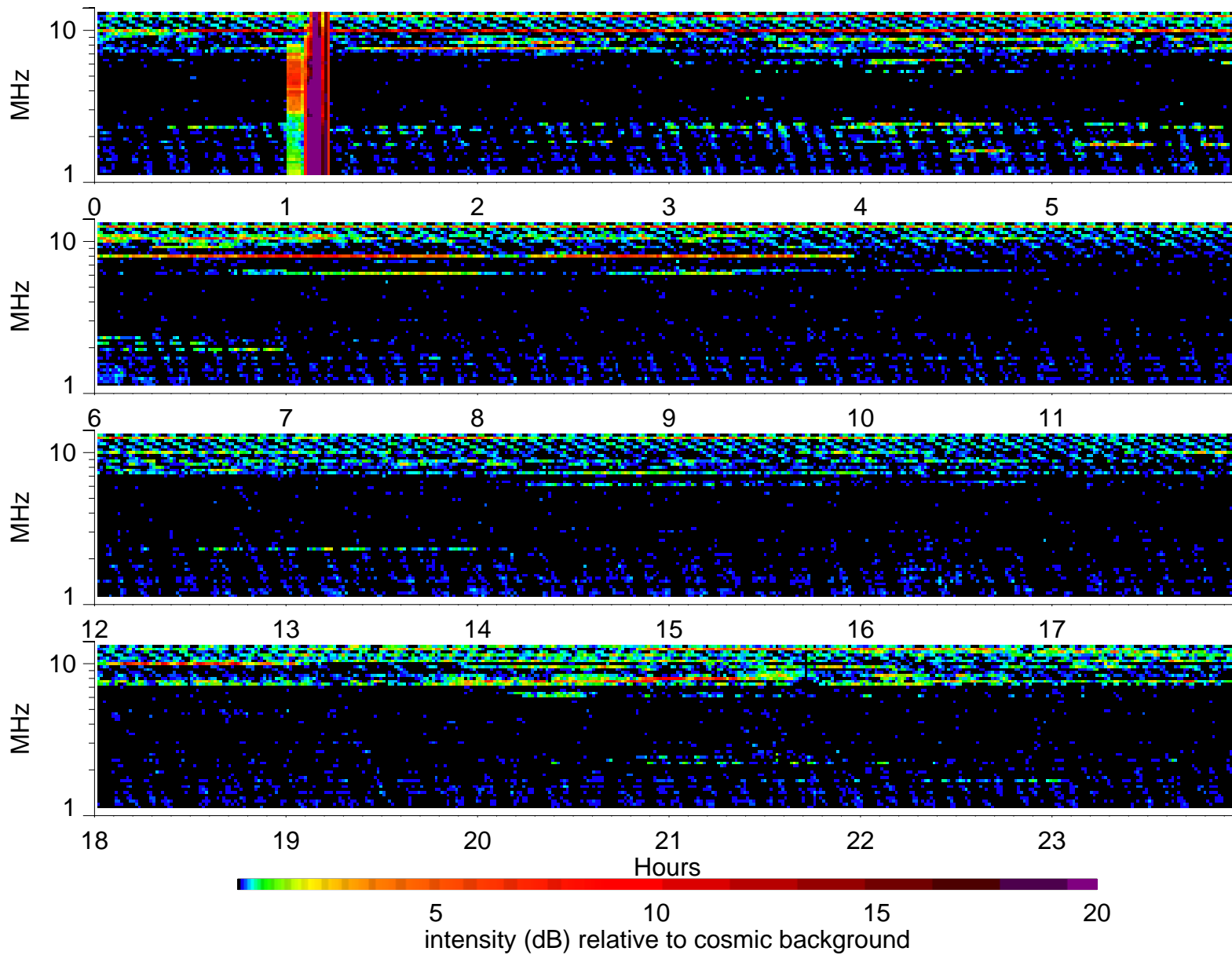
Wind Waves RAD2 receiver: 1996/10/20
