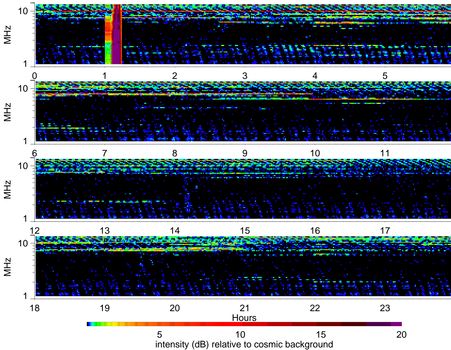
Wind Waves RAD2 receiver: 1996/10/18
