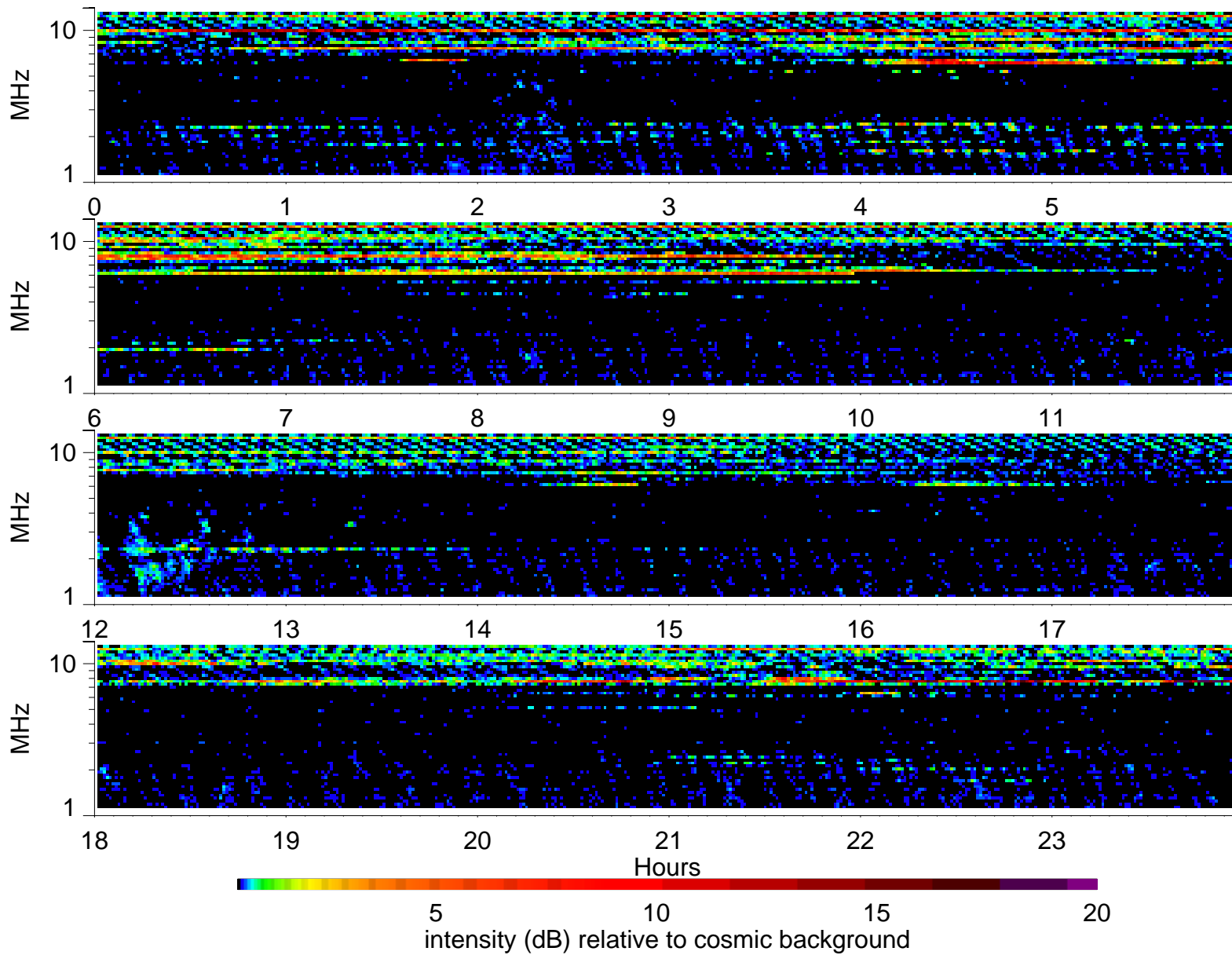
Wind Waves RAD2 receiver: 1996/10/17
