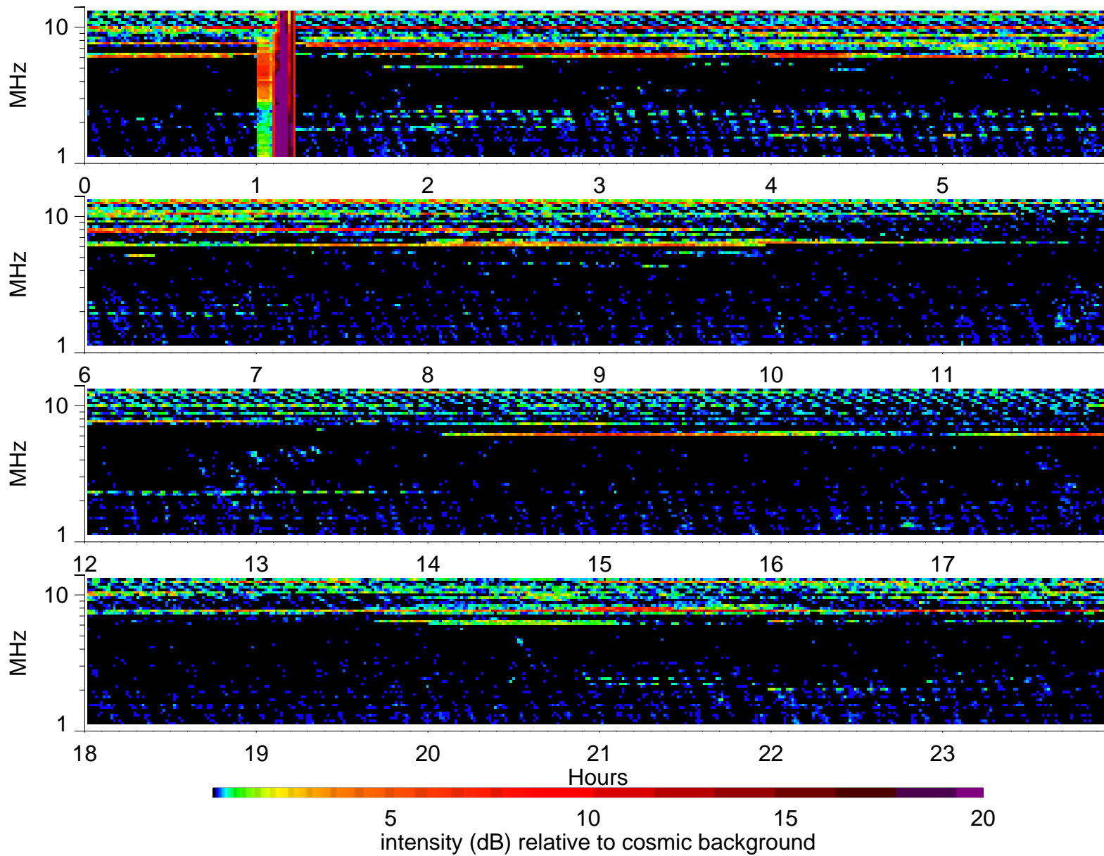
Wind Waves RAD2 receiver: 1996/10/16
