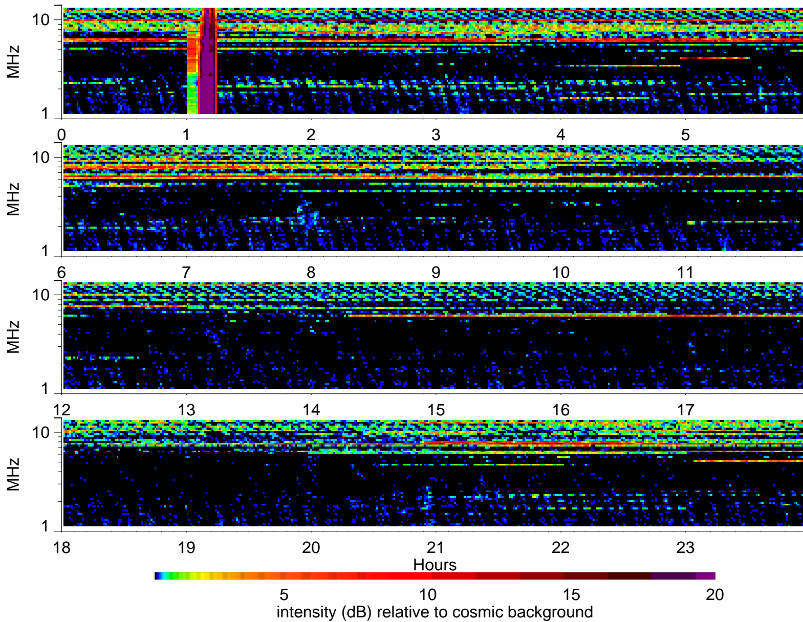
Wind Waves RAD2 receiver: 1996/10/10
