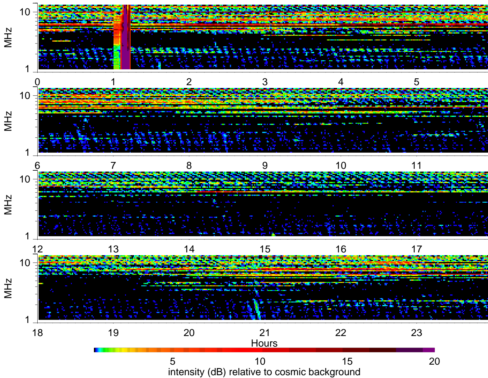
Wind Waves RAD2 receiver: 1996/10/8
