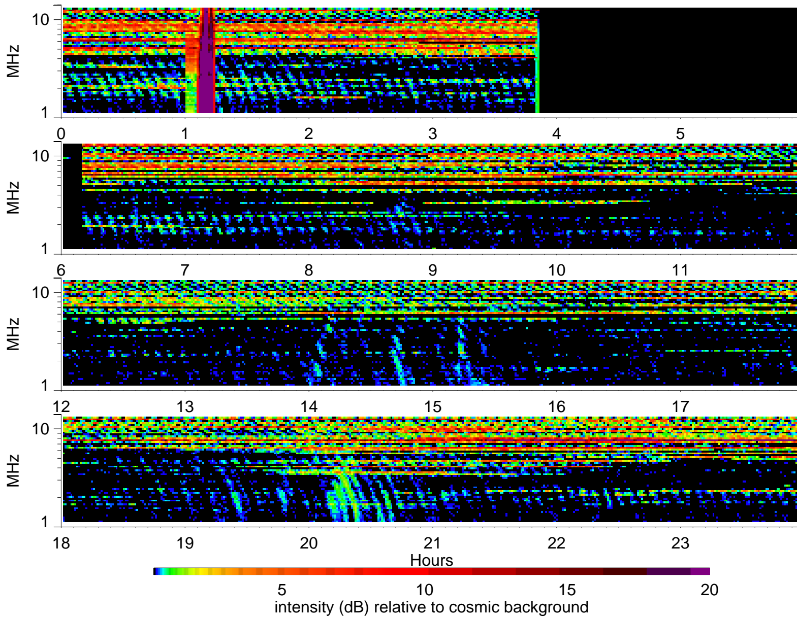
Wind Waves RAD2 receiver: 1996/10/6
