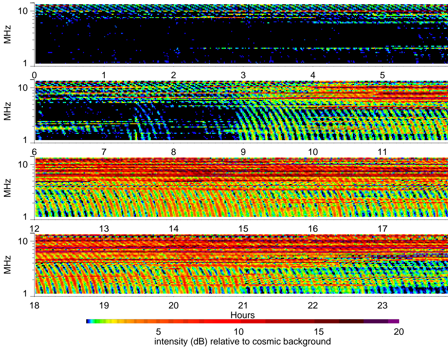
Wind Waves RAD2 receiver: 1996/10/4
