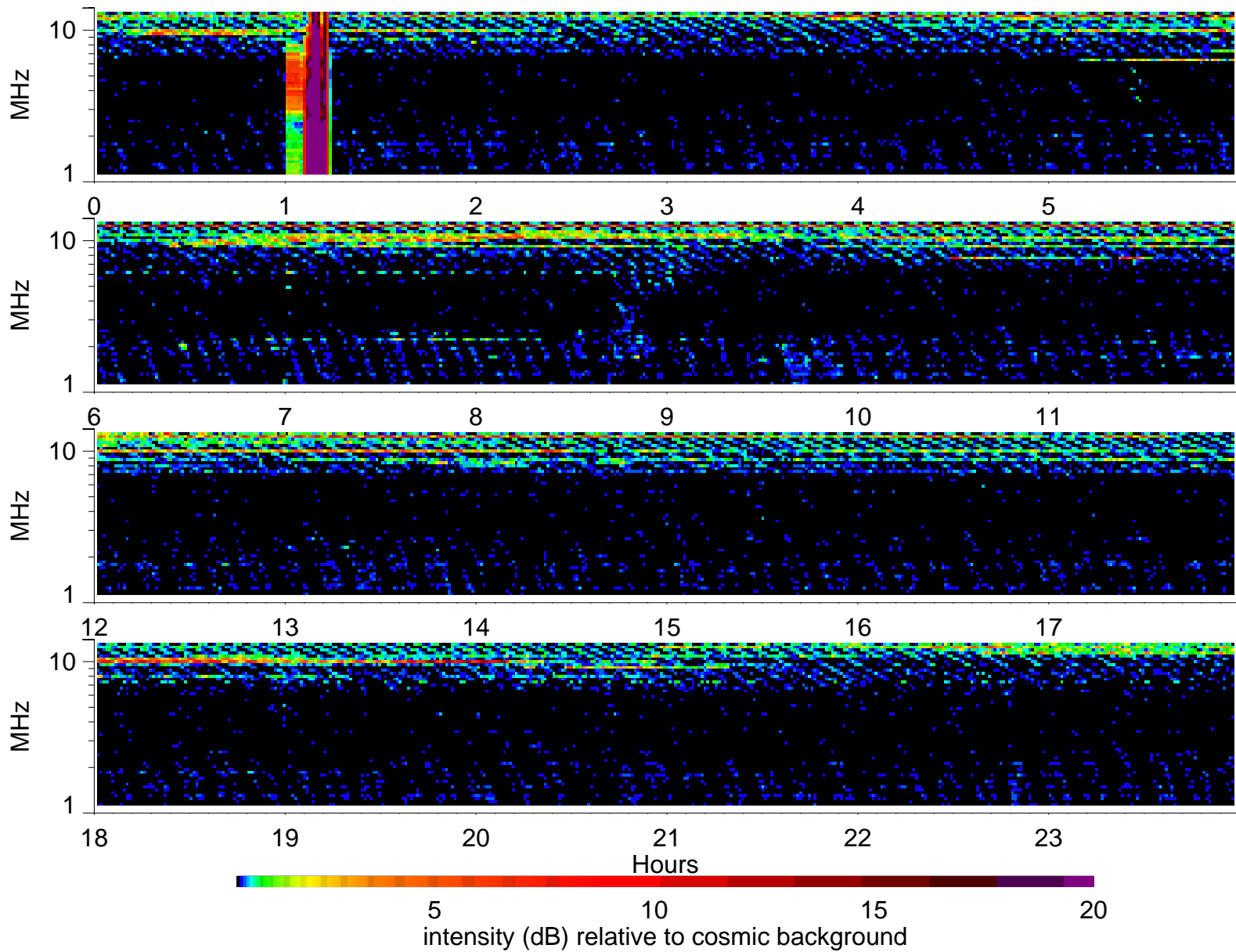
Wind Waves RAD2 receiver: 1996/9/30
