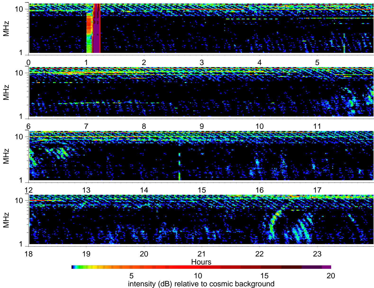
Wind Waves RAD2 receiver: 1996/9/28
