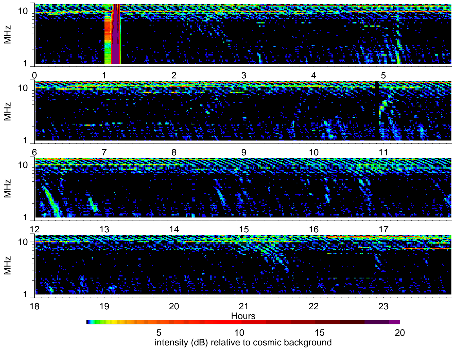
Wind Waves RAD2 receiver: 1996/9/26
