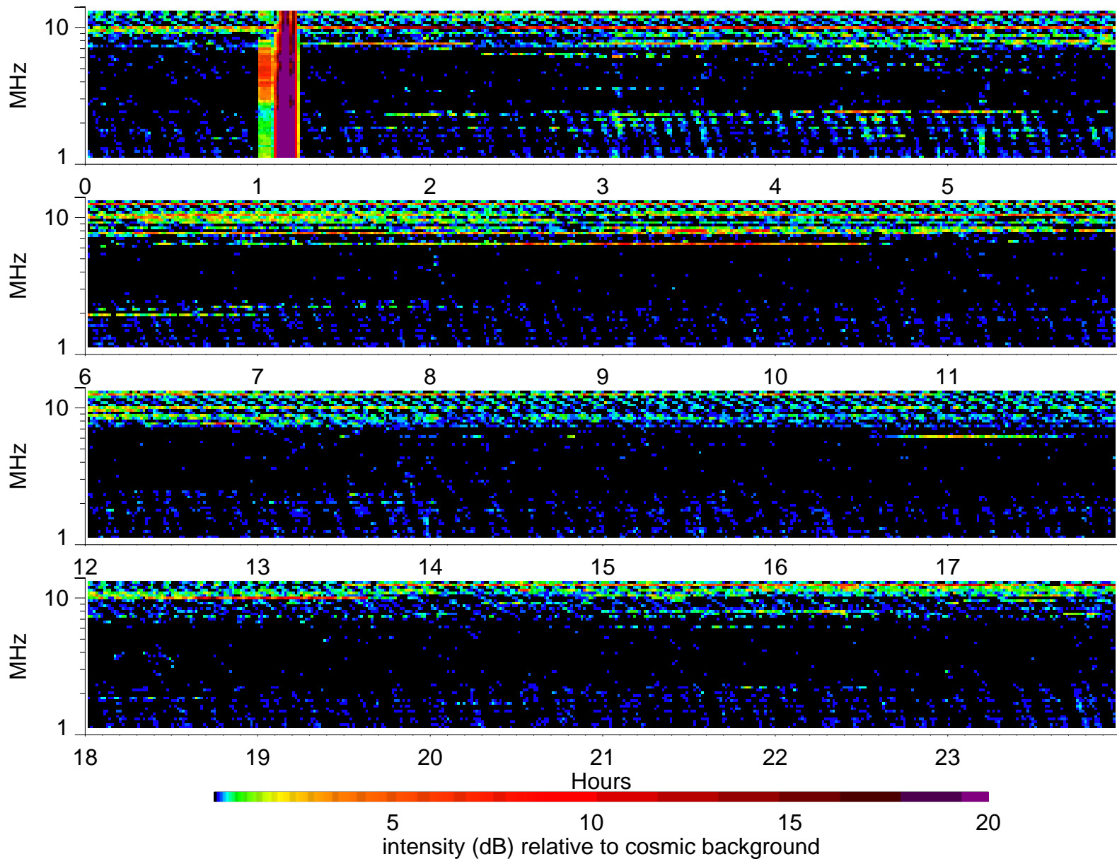
Wind Waves RAD2 receiver: 1996/9/22
