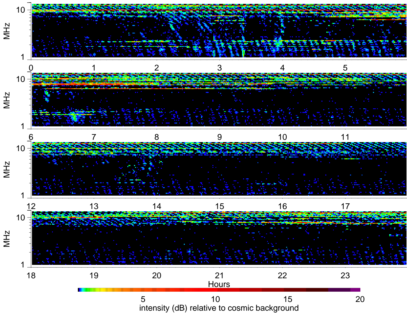
Wind Waves RAD2 receiver: 1996/9/21
