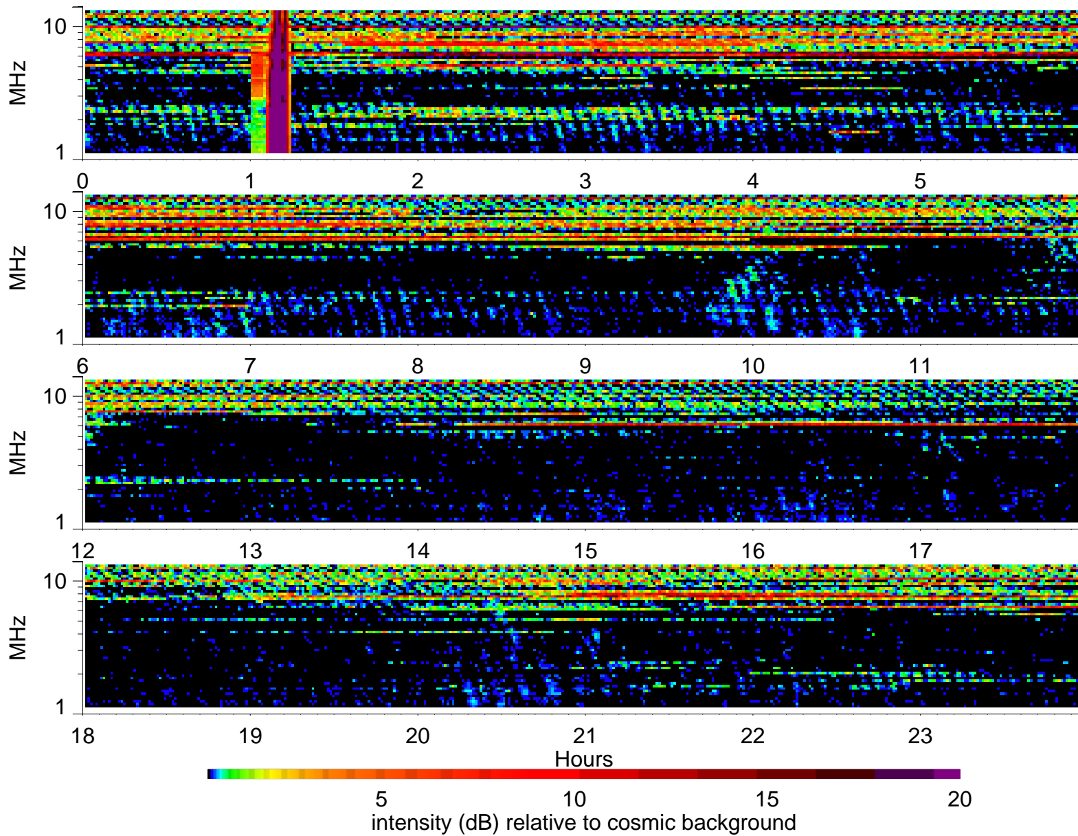
Wind Waves RAD2 receiver: 1996/9/14
