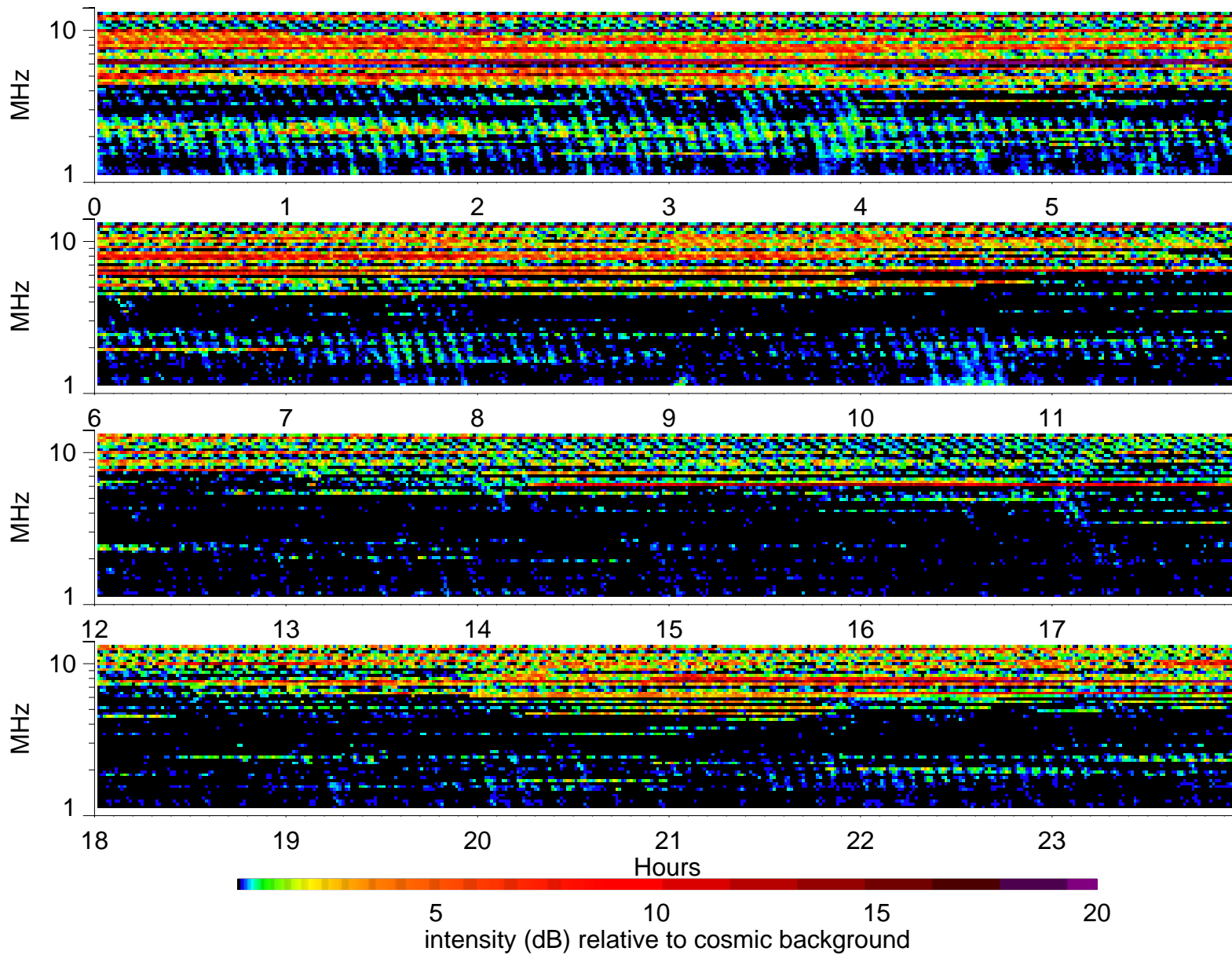
Wind Waves RAD2 receiver: 1996/9/13
