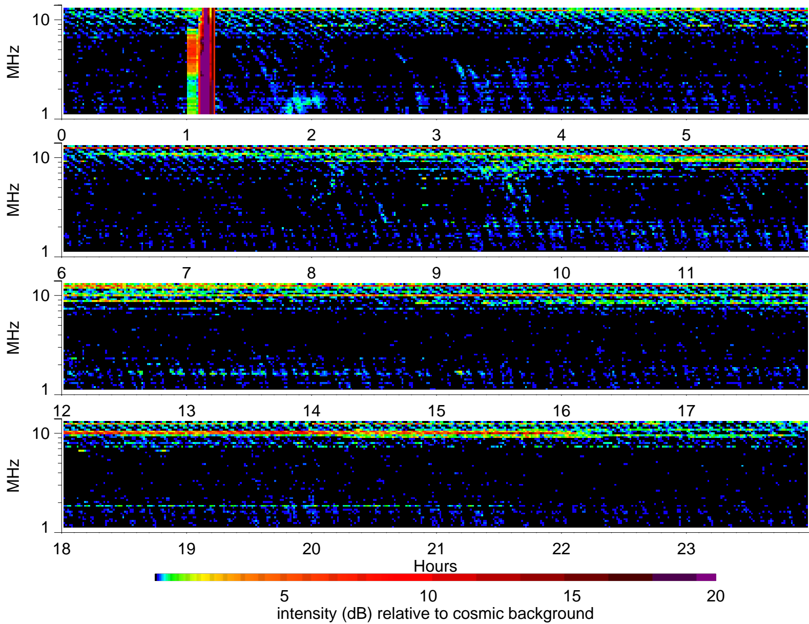
Wind Waves RAD2 receiver: 1996/9/8
