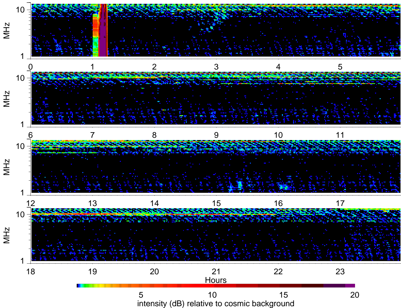
Wind Waves RAD2 receiver: 1996/9/2
