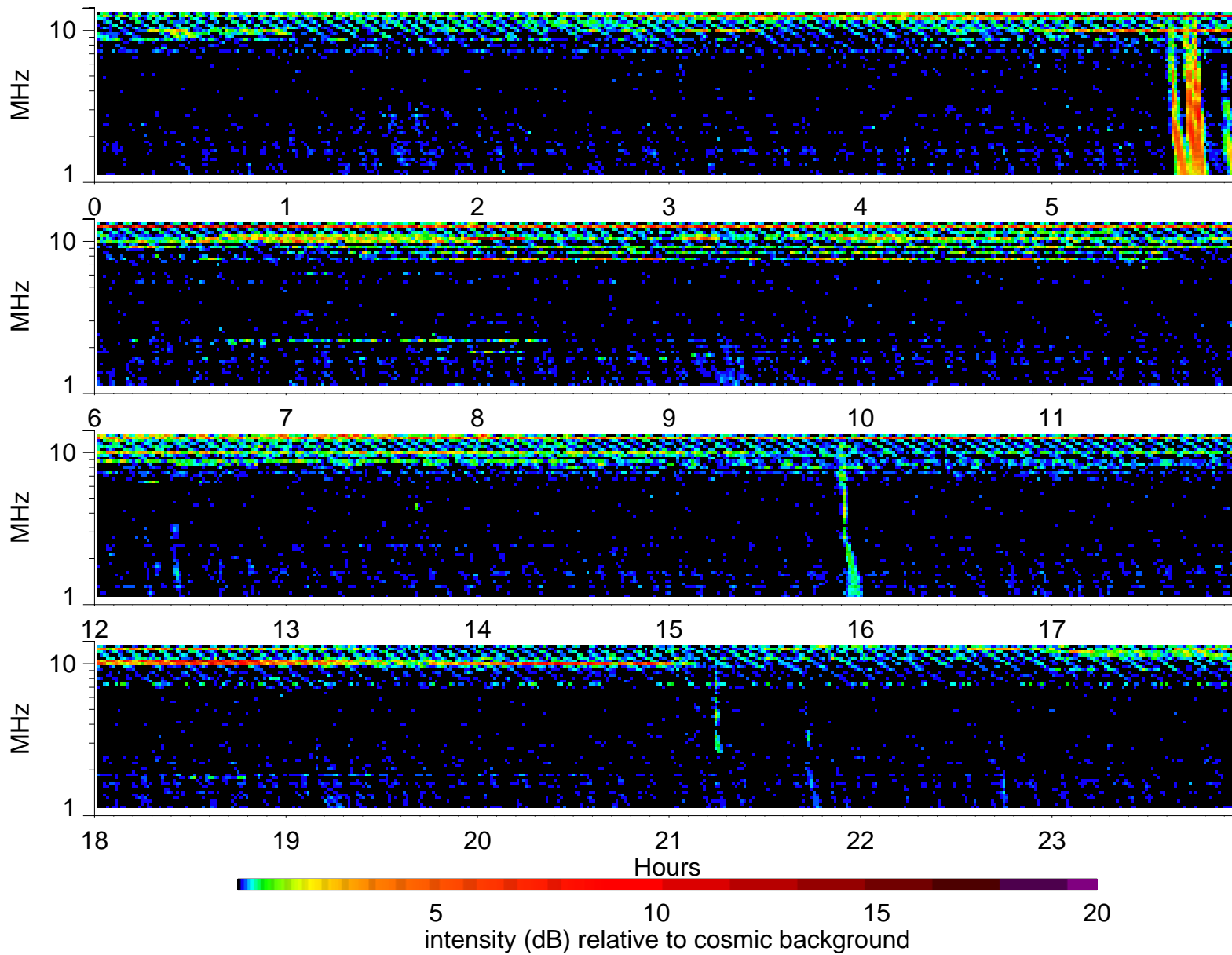
Wind Waves RAD2 receiver: 1996/8/30
