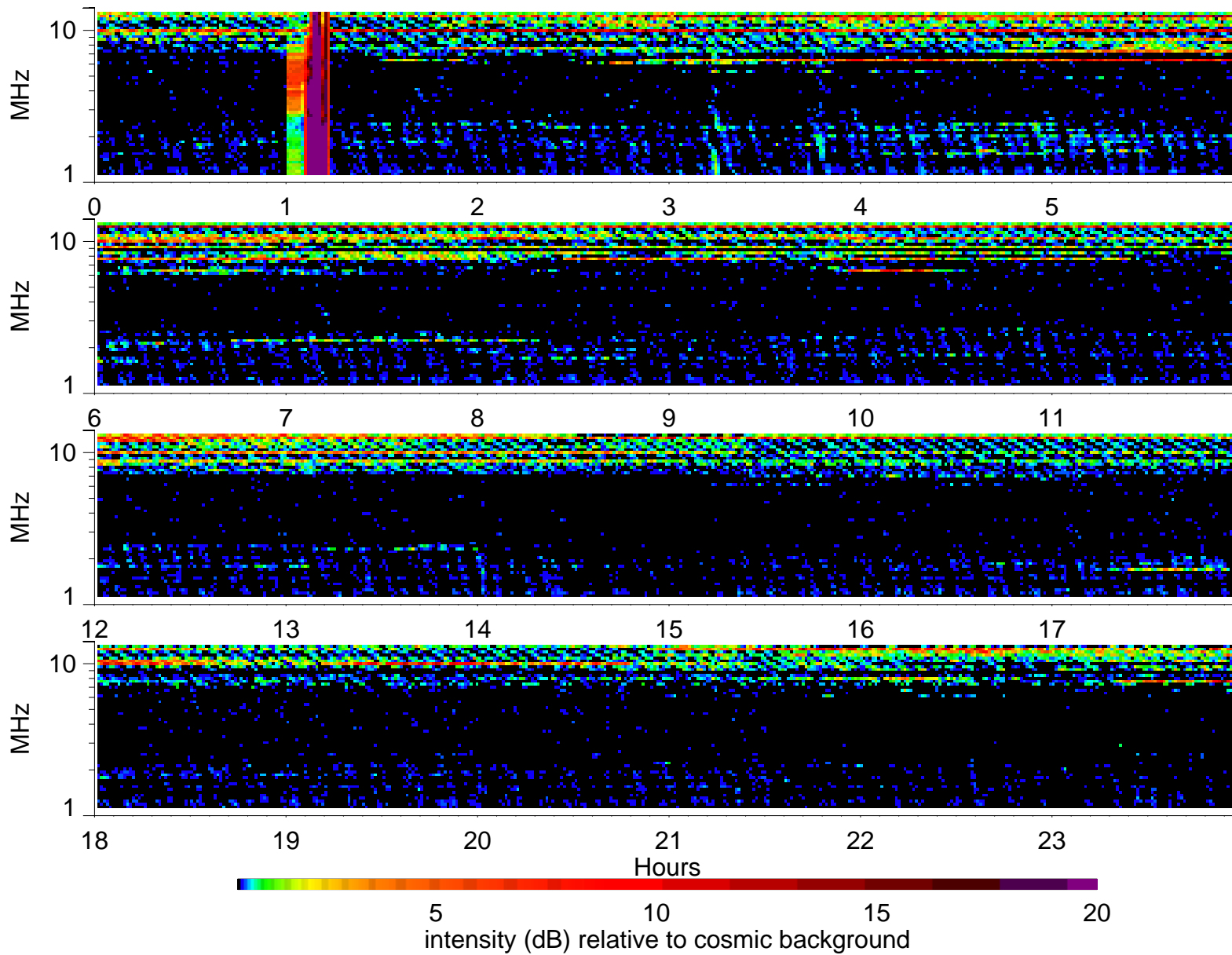
Wind Waves RAD2 receiver: 1996/8/23
