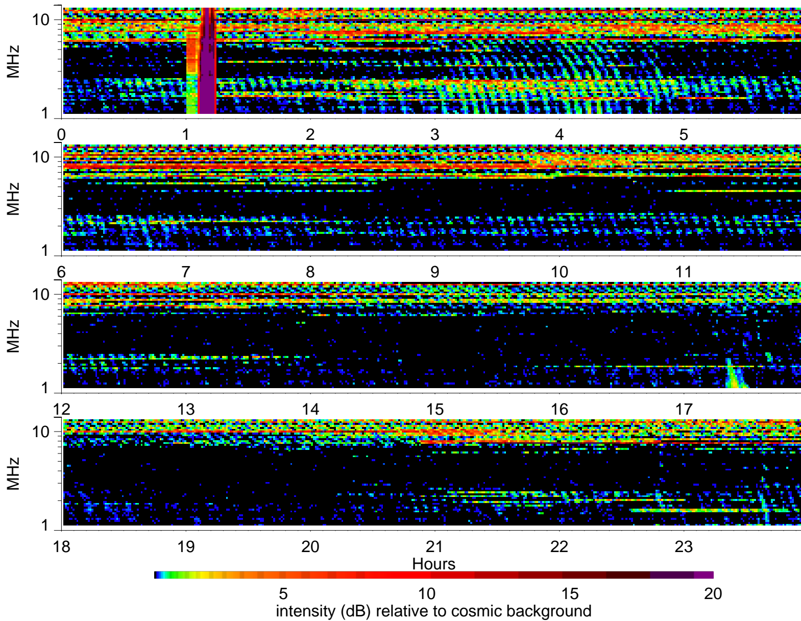
Wind Waves RAD2 receiver: 1996/8/21
