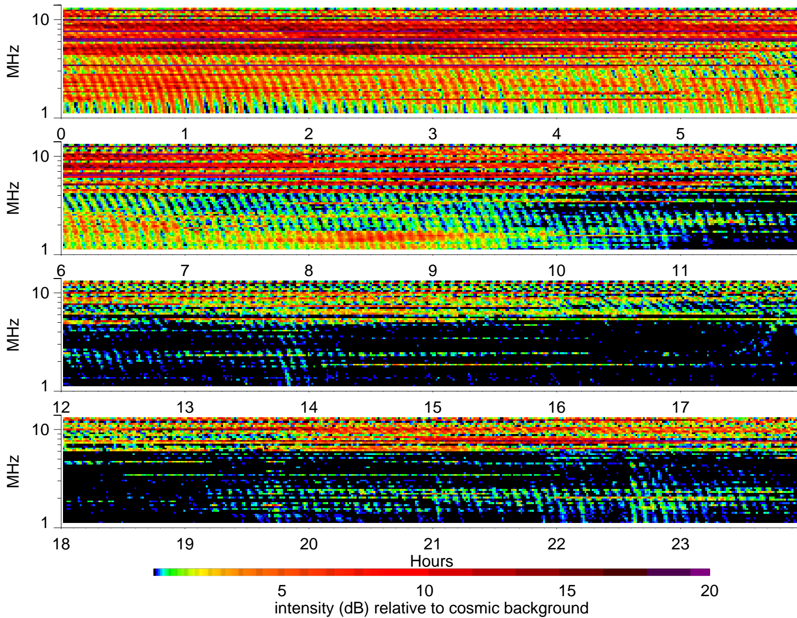
Wind Waves RAD2 receiver: 1996/8/20
