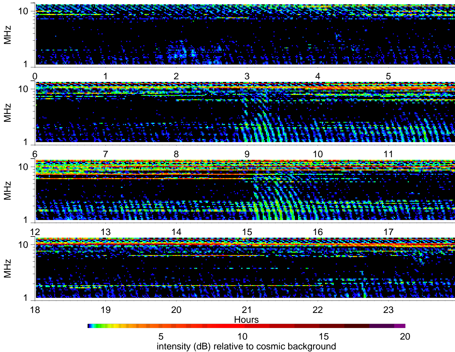
Wind Waves RAD2 receiver: 1996/8/18
