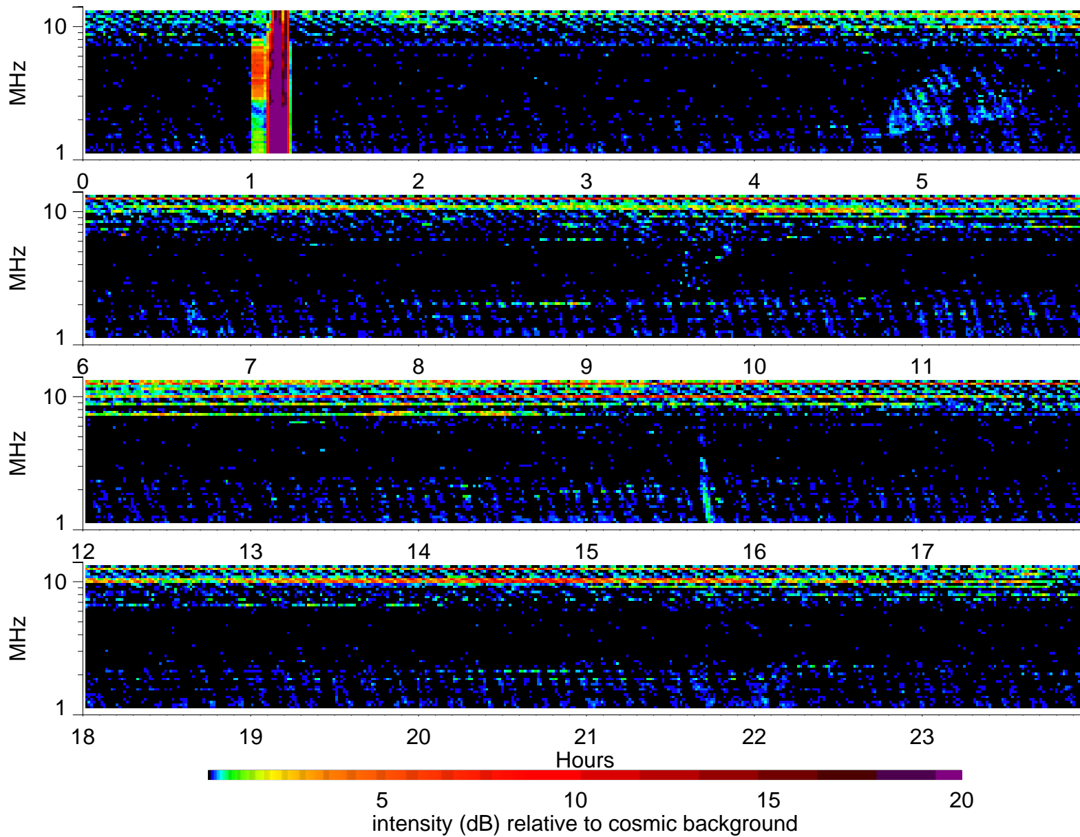
Wind Waves RAD2 receiver: 1996/8/15
