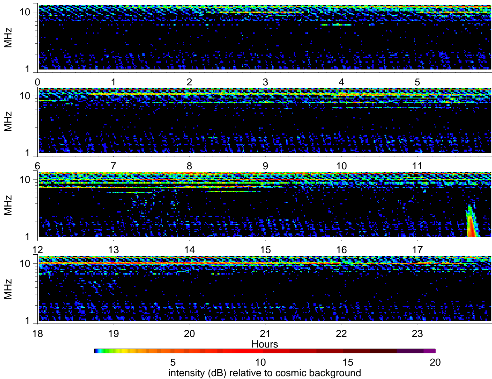
Wind Waves RAD2 receiver: 1996/8/14
