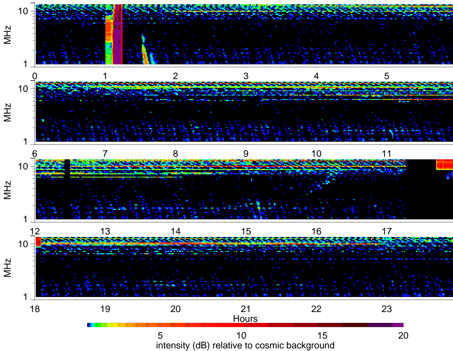
Wind Waves RAD2 receiver: 1996/8/13
