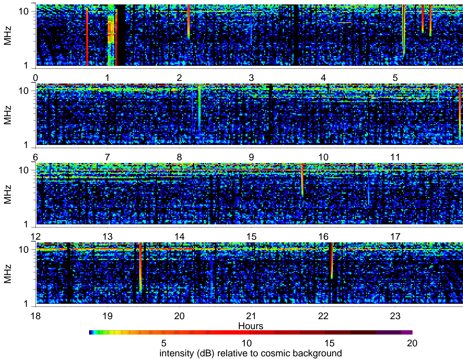
Wind Waves RAD2 receiver: 1996/8/11
