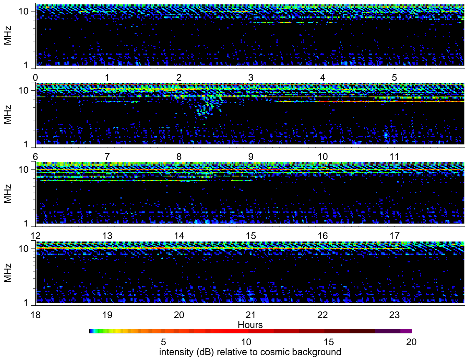
Wind Waves RAD2 receiver: 1996/8/8
